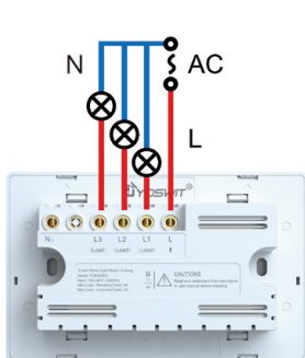
Connection 1: Without neutral wire
