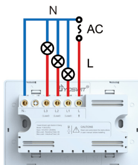
Connection 2: With neutral wire
